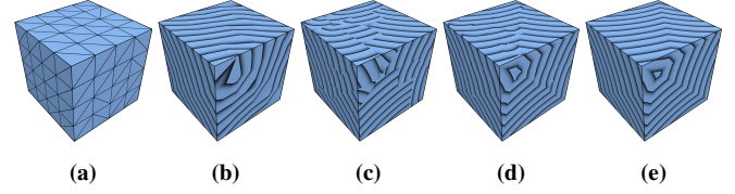
Figure 7: Geodesic distances for a tessellated cube. The source is on the back side. (b) shows linear interpolation of vertex distances. In (c), the per-triangle virtual source is used to compute the distances. The transition between different virtual sources can be refined by also considering neighboring triangles (d). Exact result is shown in (e).
