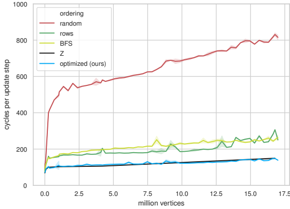
Figure 4: Cost of GSP on different memory layouts across different sizes measured in cycles per update step. Standard deviation over multiple runs is shown shaded. The test mesh is a grid. See Section 4.3 for a description of the different layouts. Our layout algorithm performs as well as the Z-order curve, which is only well defined for power-of-two grid sizes. Note that in all cases the executed instructions are the same. The only difference is the memory layout.
