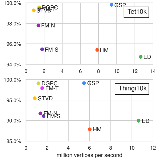
Figure 8: Accuracy (in 100% – avg error) versus throughput (in vertices per second) for different algorithms evaluated on our two test data sets. Note the different axis scales. For each mesh, the same 20 experiments with a single source located at a random vertex were performed. The compared algorithms are our GSP, Dijkstra on edge lengths (ED), the heat method (HM), fast marching from Sethian (FM-S), Novotni (FM-N), Tang (FM-T), discrete geodesic polar coordinates (DGPC), and the short-term vector Dijkstra (STVD). Box plots of performance and accuracy can be found in the supplemental material.
