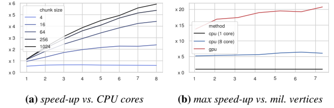
Figure 11: For large meshes or many sources, a parallel implementation of our method can lead to significant performance improvements. The first graph plots speed-up against CPU cores on a 4 million vertices mesh with 1000 sources, the second plots the largest observed speed-up against mesh size and compares CPU and GPU implementations.
